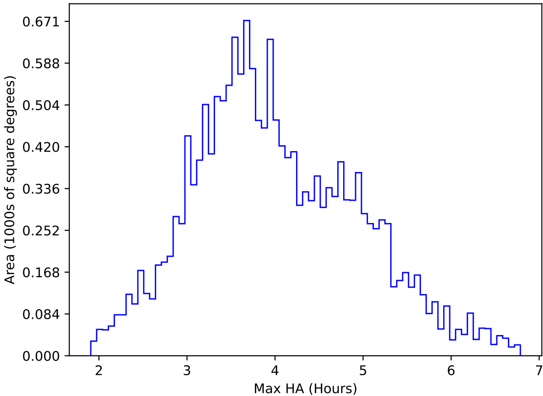
too_elab_r128_d2_griz_v3.4_10yrs WFD u band: Max HA
