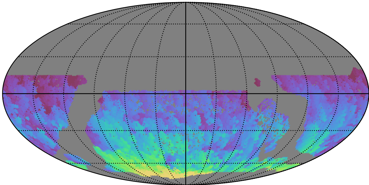
too_elab_r128_d2_griz_v3.4_10yrs WFD r band: Max HA
