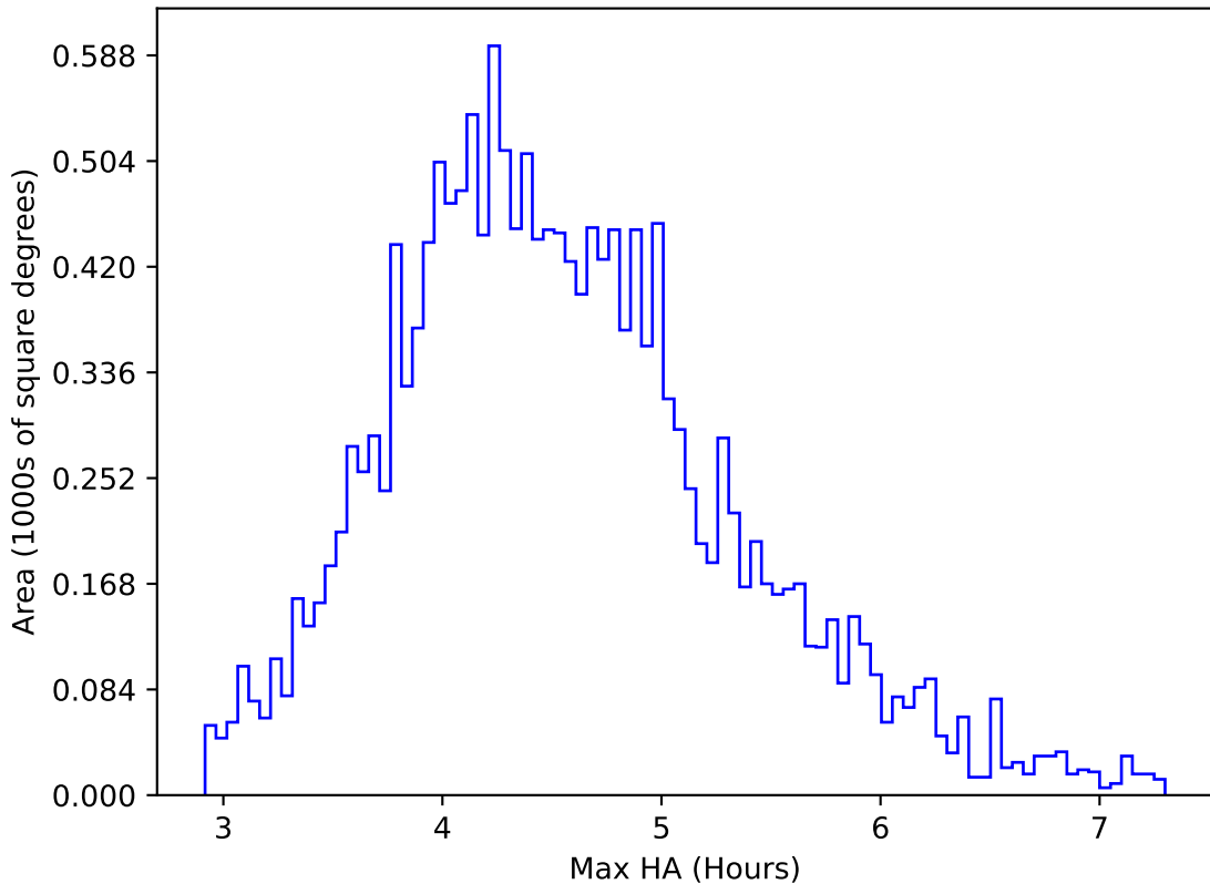
too_elab_r128_d2_griz_v3.4_10yrs WFD r band: Max HA
