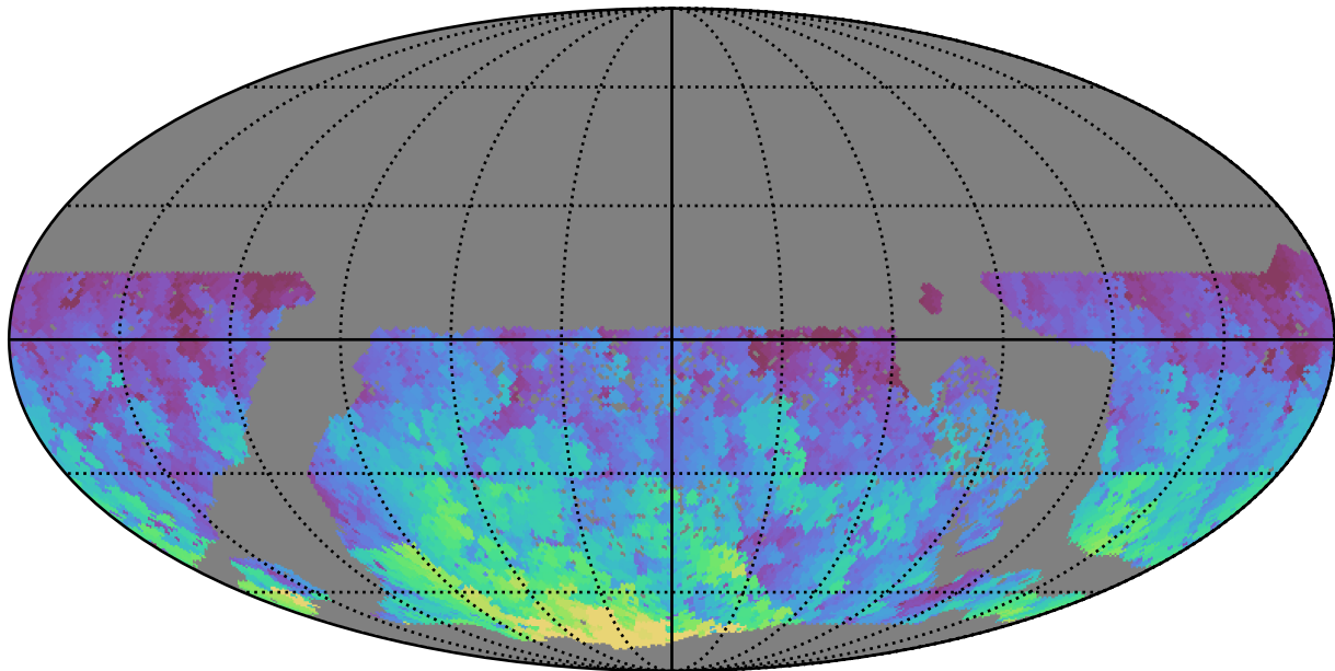
too_elab_r128_d2_griz_v3.4_10yrs WFD g band: Max HA
