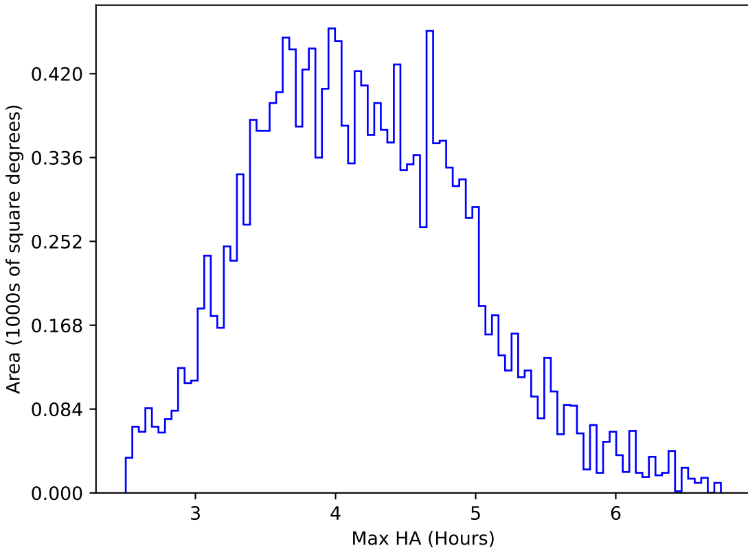
too_elab_r128_d2_griz_v3.4_10yrs WFD g band: Max HA
