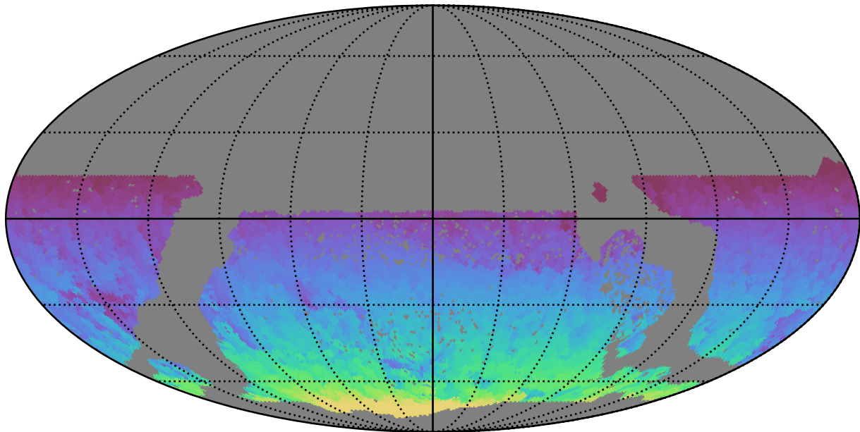
too_elab_r128_d2_griz_v3.4_10yrs WFD all bands: Max HA
