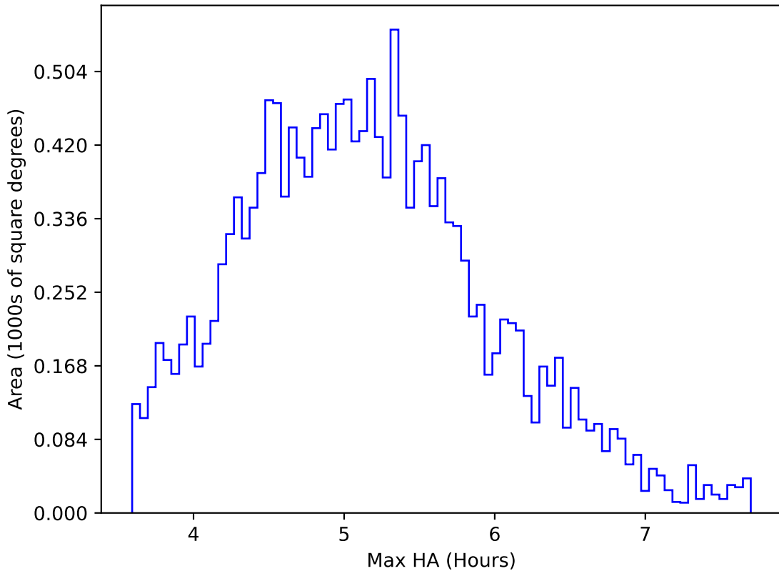
too_elab_r128_d2_griz_v3.4_10yrs WFD all bands: Max HA
