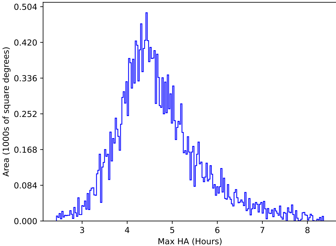
too_elab_r128_d2_griz_v3.4_10yrs All sky y band: Max HA
