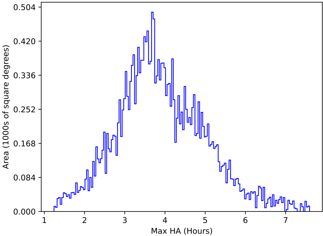
too_elab_r128_d2_griz_v3.4_10yrs All sky u band: Max HA
