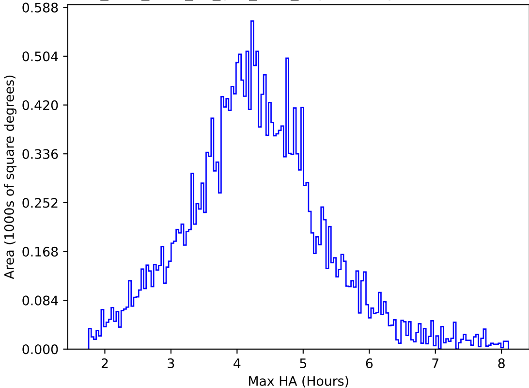
too_elab_r128_d2_griz_v3.4_10yrs All sky r band: Max HA
