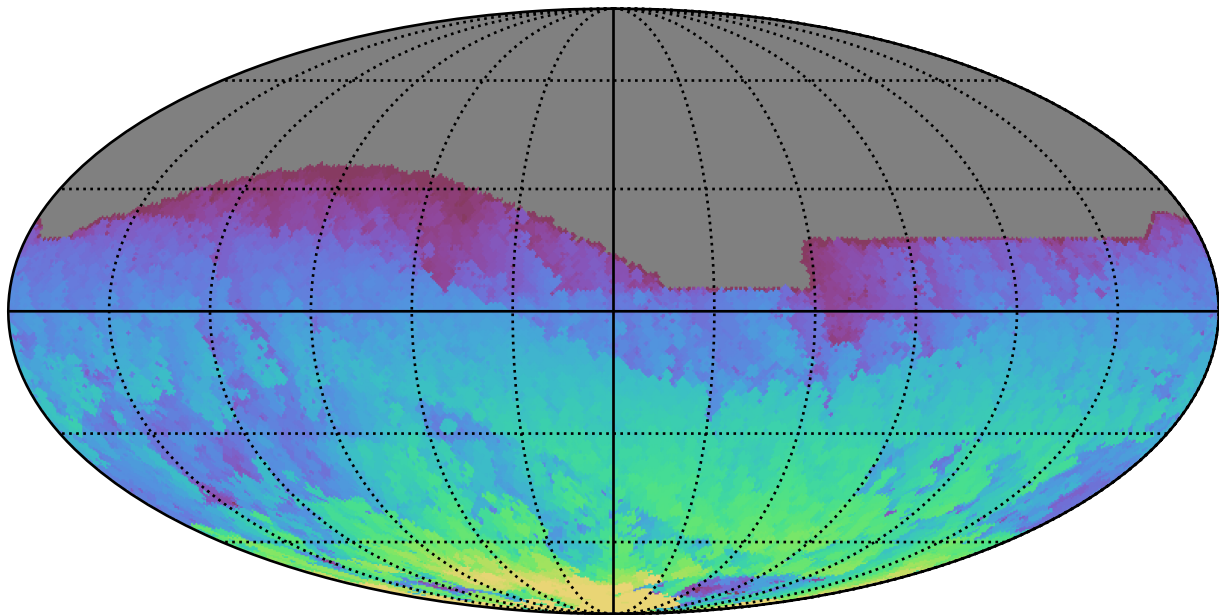
too_elab_r128_d2_griz_v3.4_10yrs All sky i band: Max HA
