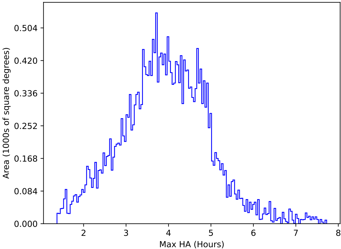
too_elab_r128_d2_griz_v3.4_10yrs All sky g band: Max HA
