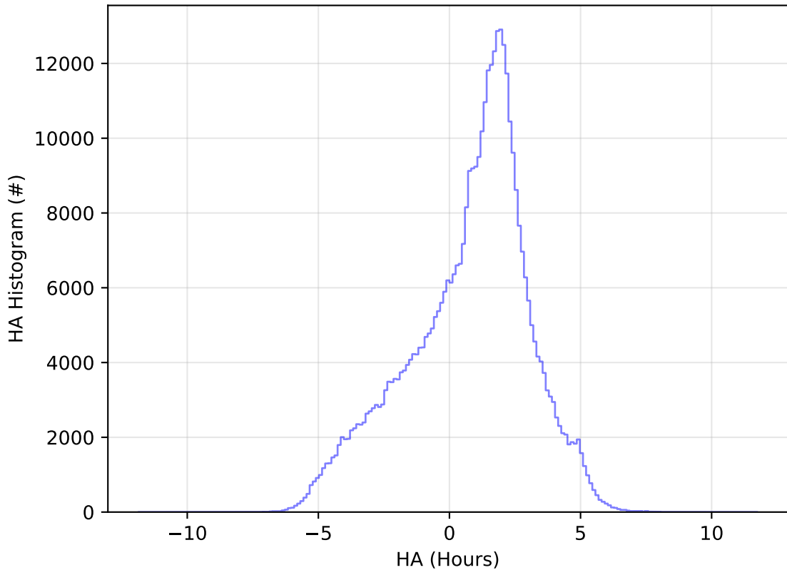
too_elab_r128_d2_griz_v3.4_10yrs WFD z band: HA Histogram
