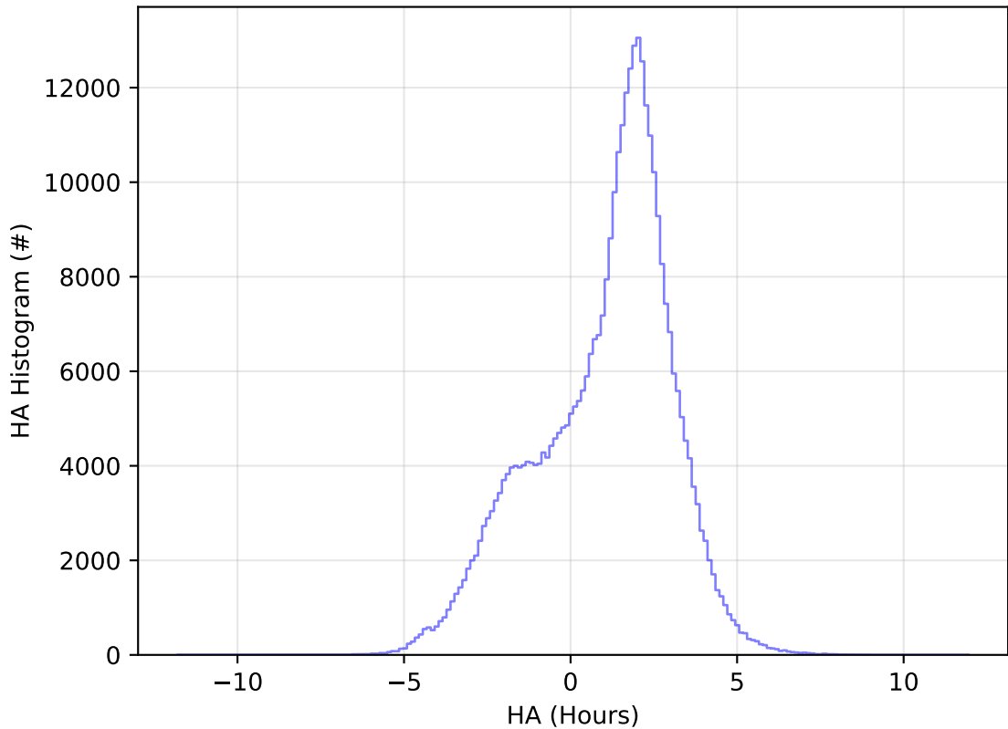
too_elab_r128_d2_griz_v3.4_10yrs WFD y band: HA Histogram
