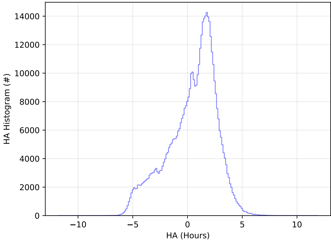
too_elab_r128_d2_griz_v3.4_10yrs WFD r band: HA Histogram
