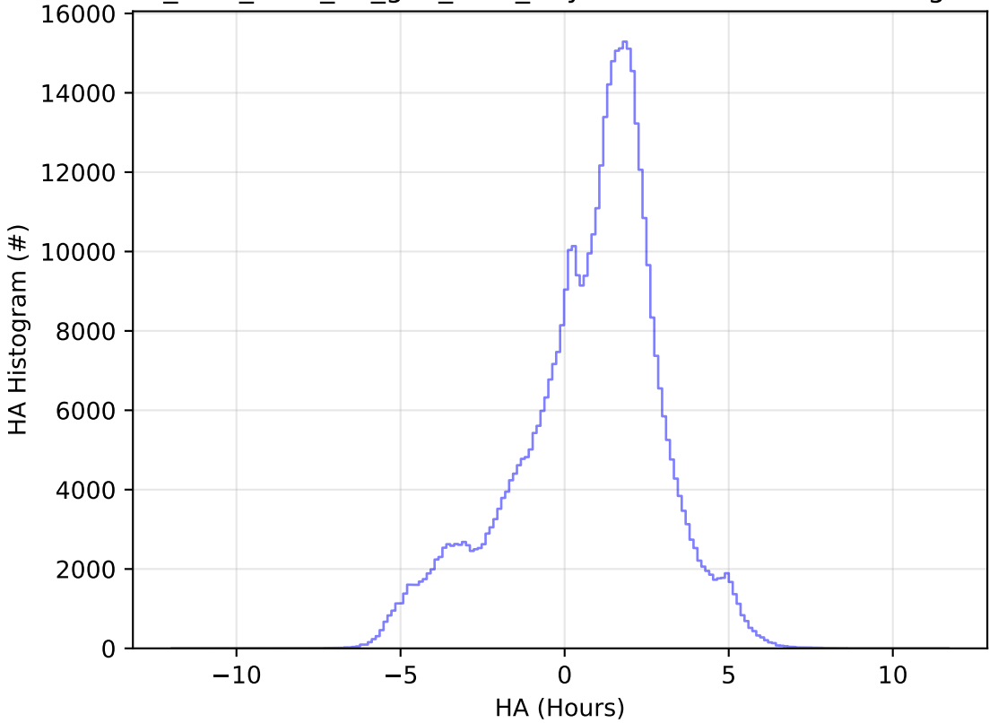
too_elab_r128_d2_griz_v3.4_10yrs WFD i band: HA Histogram
