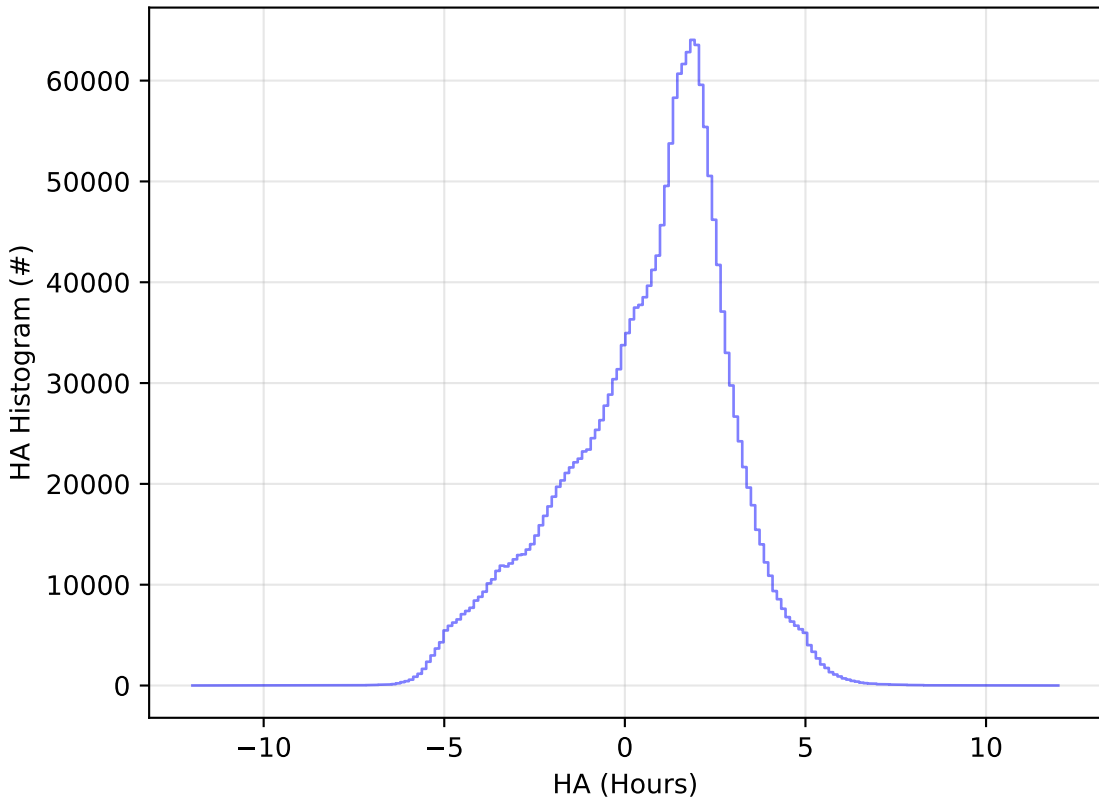
too_elab_r128_d2_griz_v3.4_10yrs WFD all bands: HA Histogram
