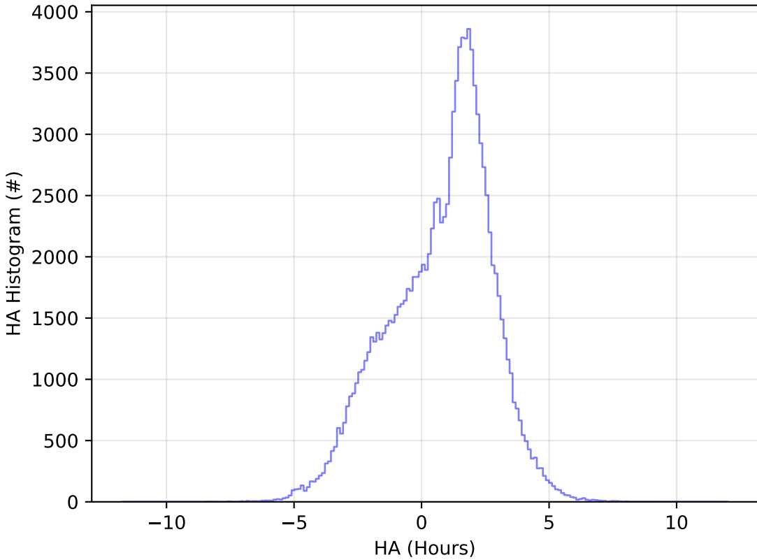
too_elab_r128_d2_griz_v3.4_10yrs All sky u band: HA Histogram
