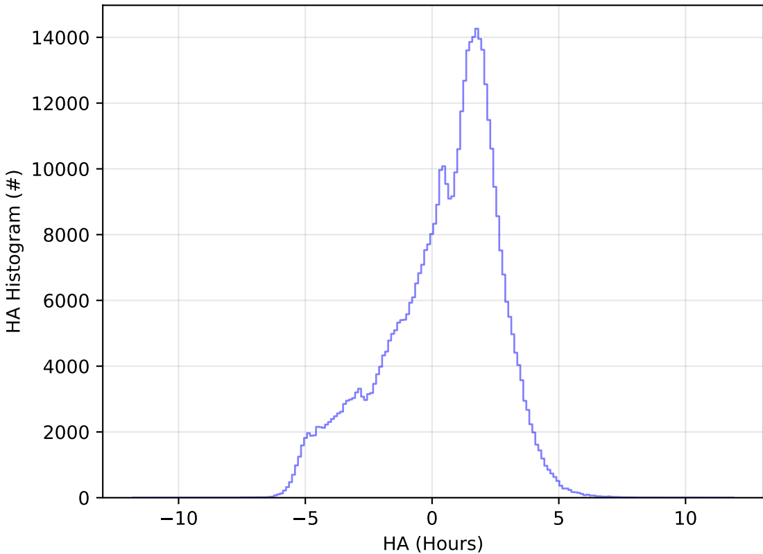
too_elab_r128_d2_griz_v3.4_10yrs All sky r band: HA Histogram
