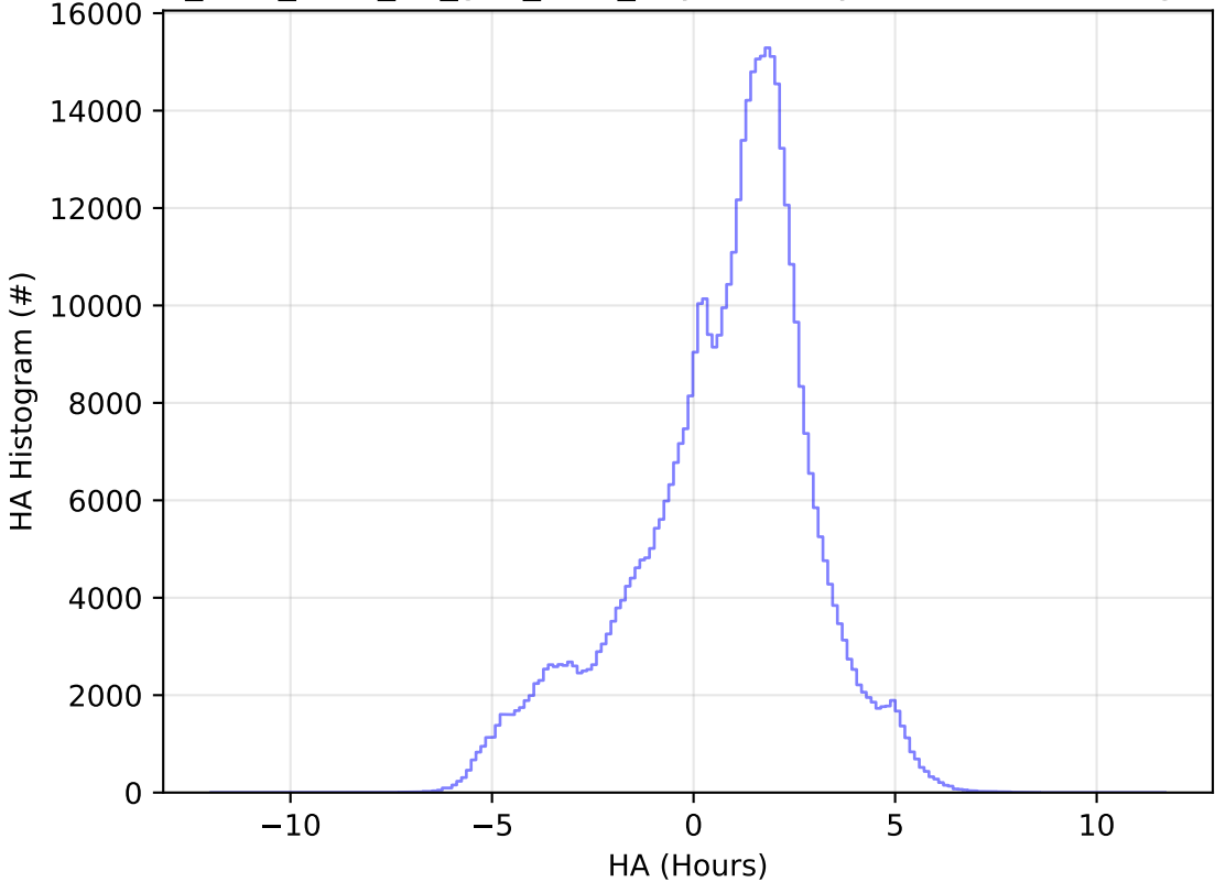
too_elab_r128_d2_griz_v3.4_10yrs All sky i band: HA Histogram
