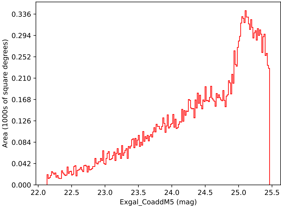
too_elab_r128_d2_griz_v3.4_10yrs Yr 3-4 i band: Exgal_CoaddM5
