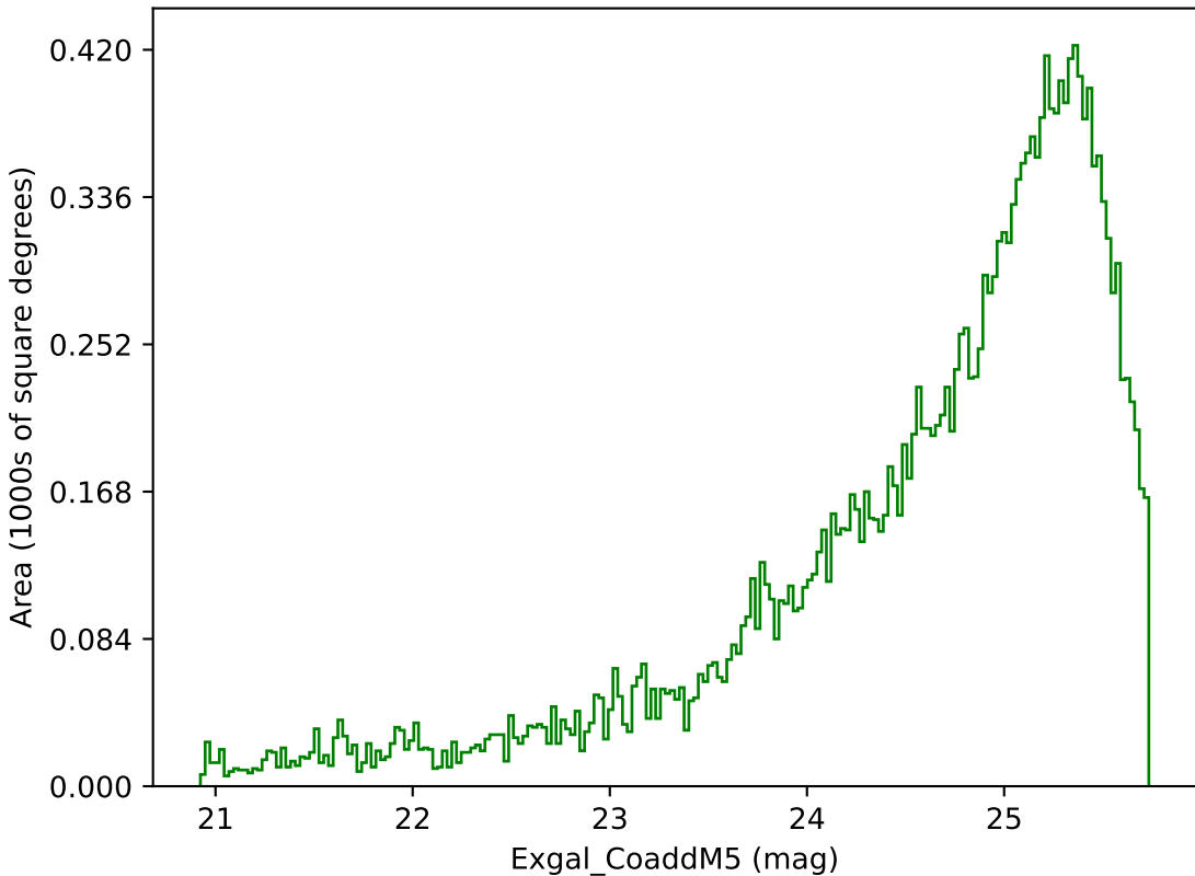
too_elab_r128_d2_griz_v3.4_10yrs Yr 3-4 g band: Exgal_CoaddM5
