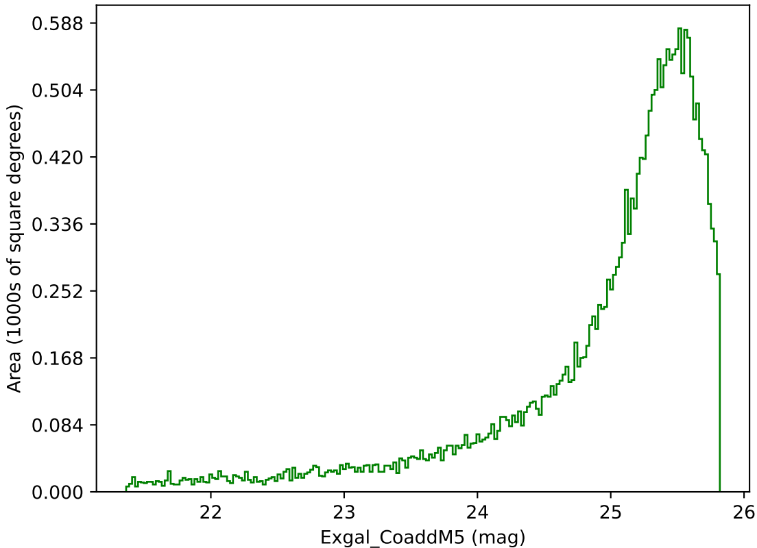
too_elab_r128_d2_griz_v3.4_10yrs Yr 1 g band: Exgal_CoaddM5
