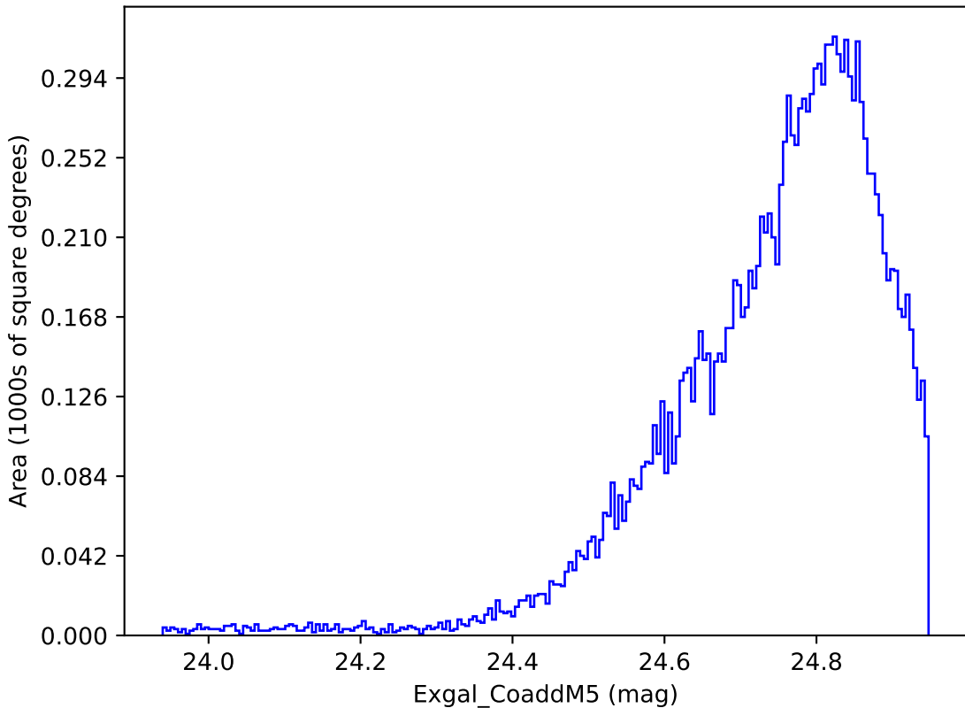
too_elab_r128_d2_griz_v3.4_10yrs WFD y band: Exgal_CoaddM5
