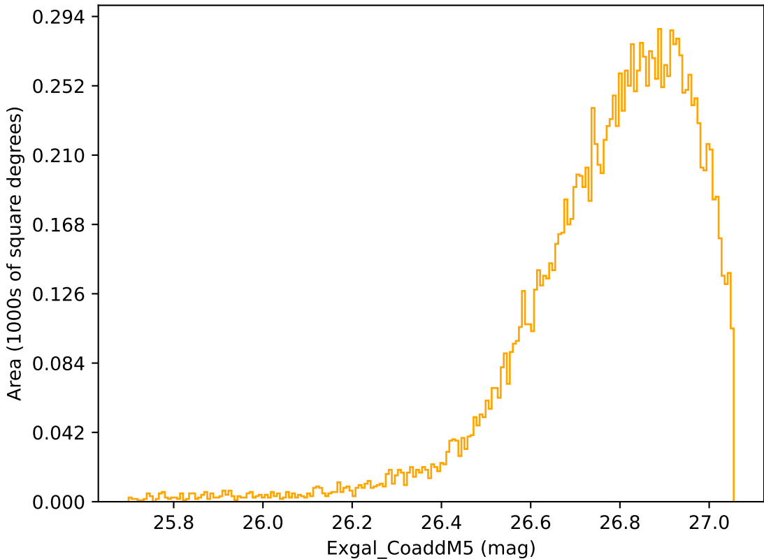
too_elab_r128_d2_griz_v3.4_10yrs WFD r band: Exgal_CoaddM5
