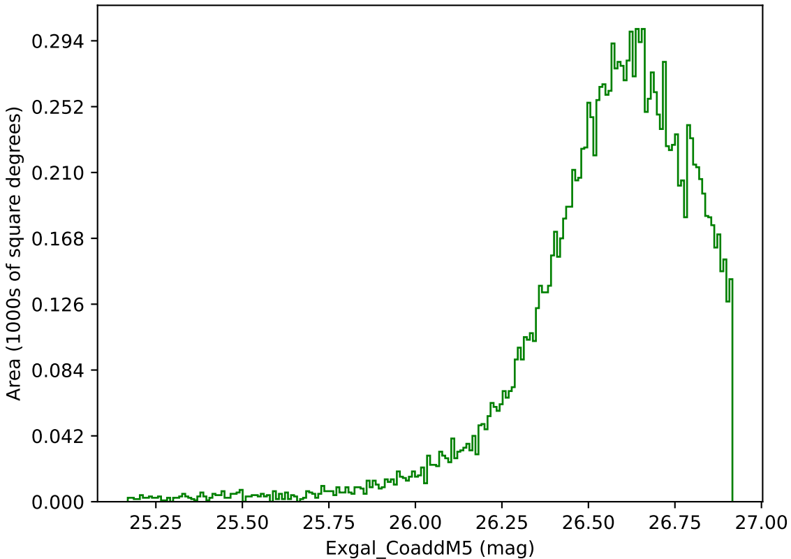
too_elab_r128_d2_griz_v3.4_10yrs WFD g band: Exgal_CoaddM5
