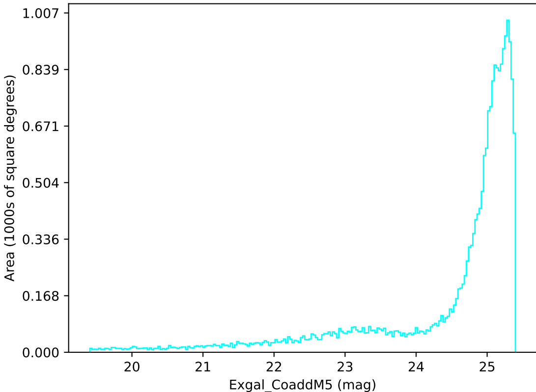
too_elab_r128_d2_griz_v3.4_10yrs All sky u band: Exgal_CoaddM5
