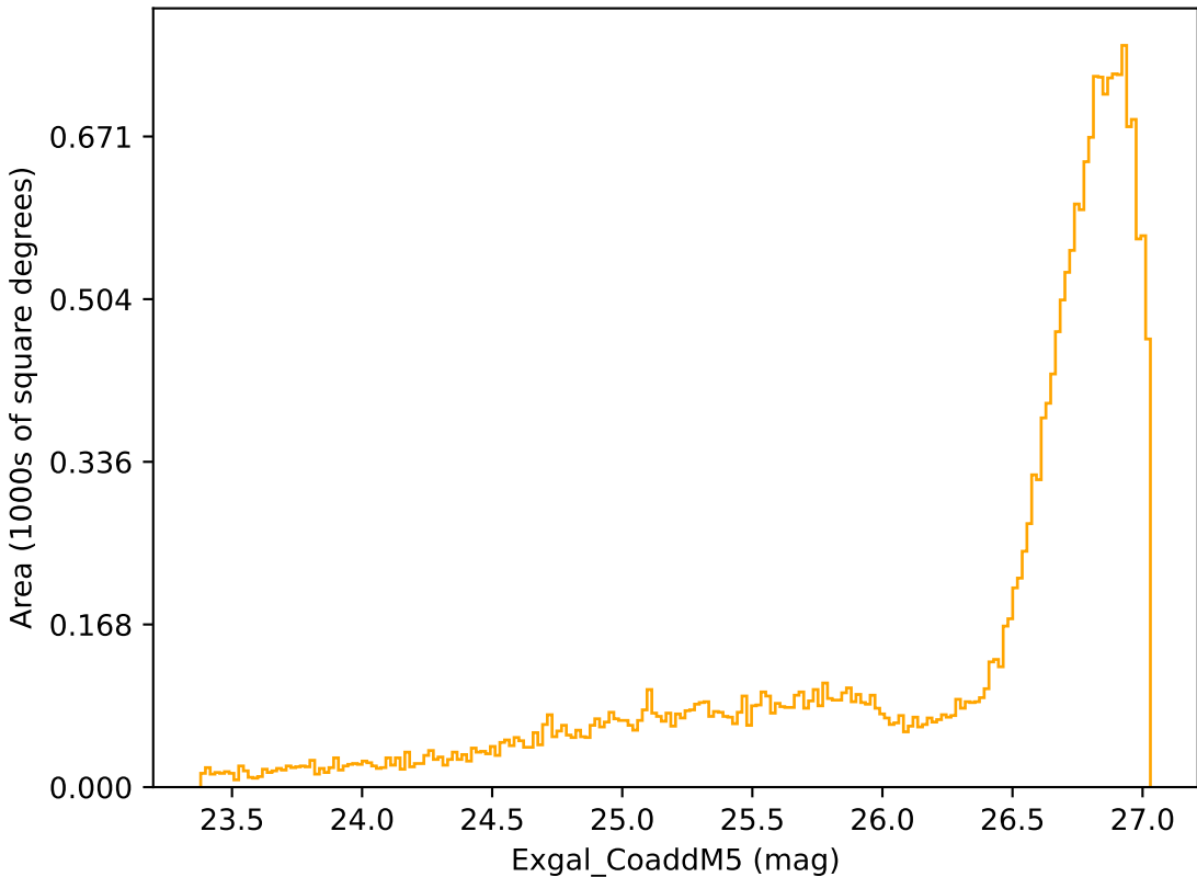
too_elab_r128_d2_griz_v3.4_10yrs All sky r band: Exgal_CoaddM5
