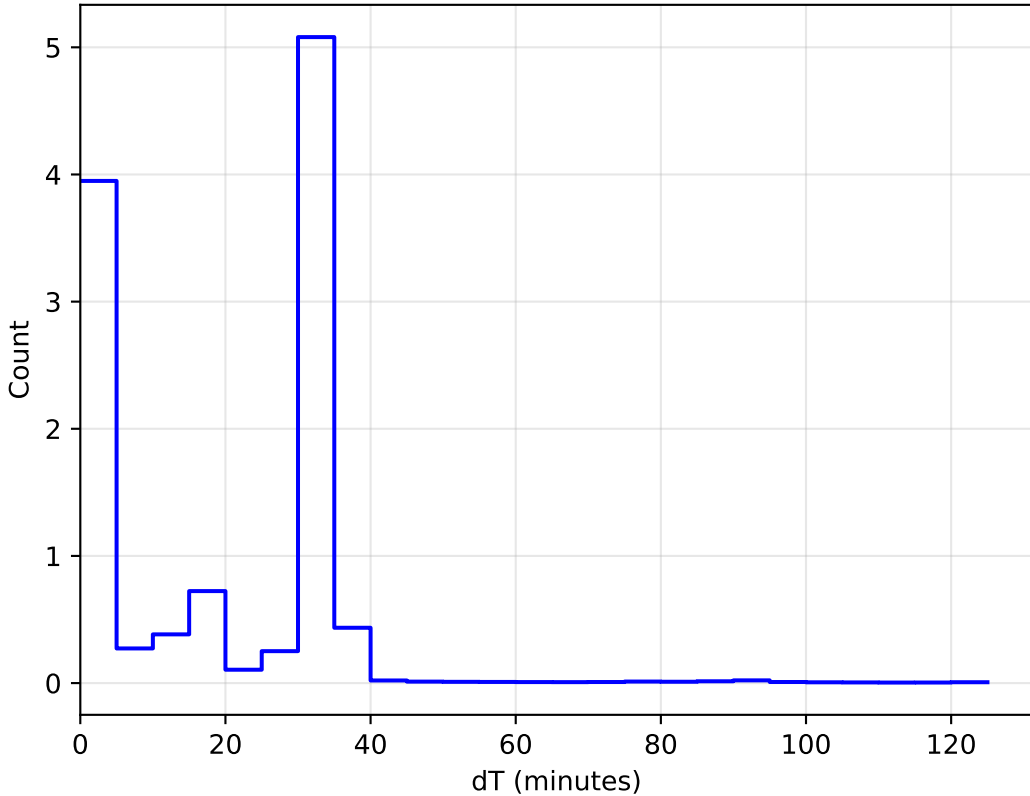
too_elab_r128_d2_griz_v3.4_10yrs WFD: DeltaT Histogram 1e6
