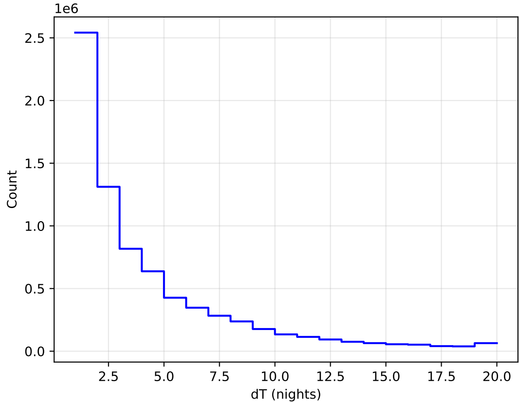
too_elab_r128_d2_griz_v3.4_10yrs WFD all bands: DeltaNight Histogram
