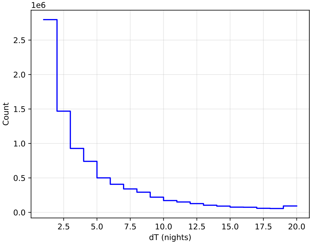
too_elab_r128_d2_griz_v3.4_10yrs All sky all bands: DeltaNight Histogram
