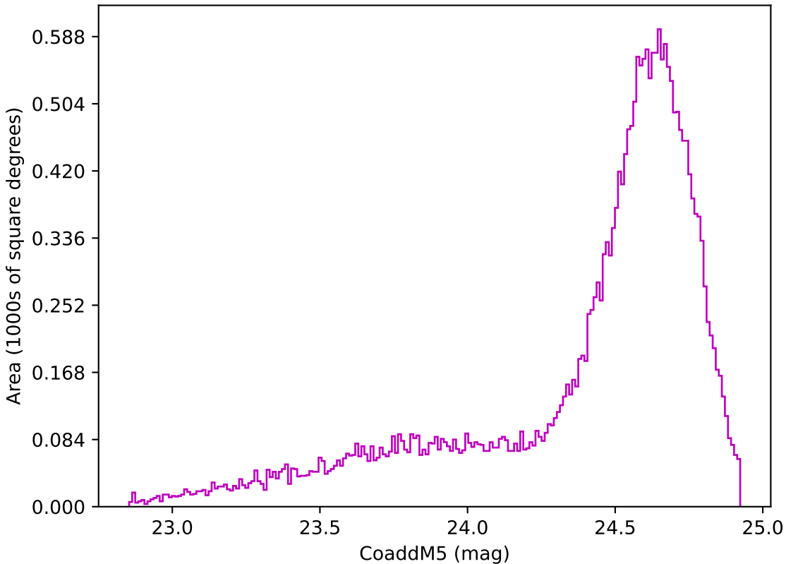
too_elab_r128_d2_griz_v3.4_10yrs Yr 1 z band: CoaddM5
