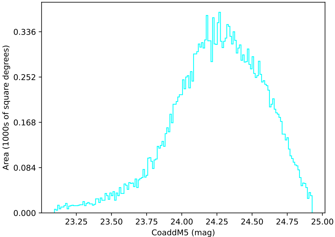
too_elab_r128_d2_griz_v3.4_10yrs Yr 1 u band: CoaddM5
