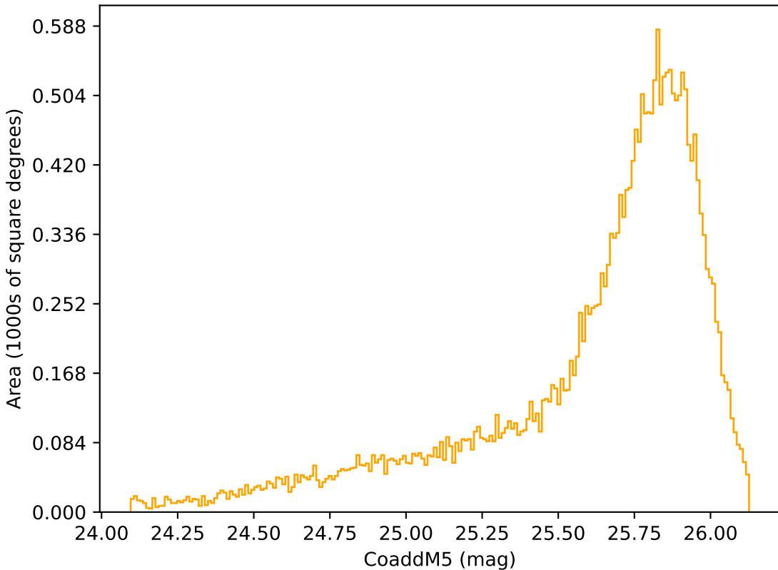
too_elab_r128_d2_griz_v3.4_10yrs Yr 1 r band: CoaddM5
