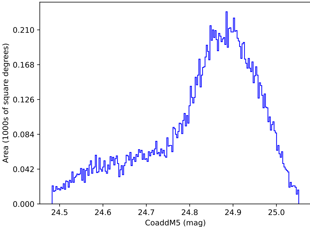
too_elab_r128_d2_griz_v3.4_10yrs WFD y band: CoaddM5
