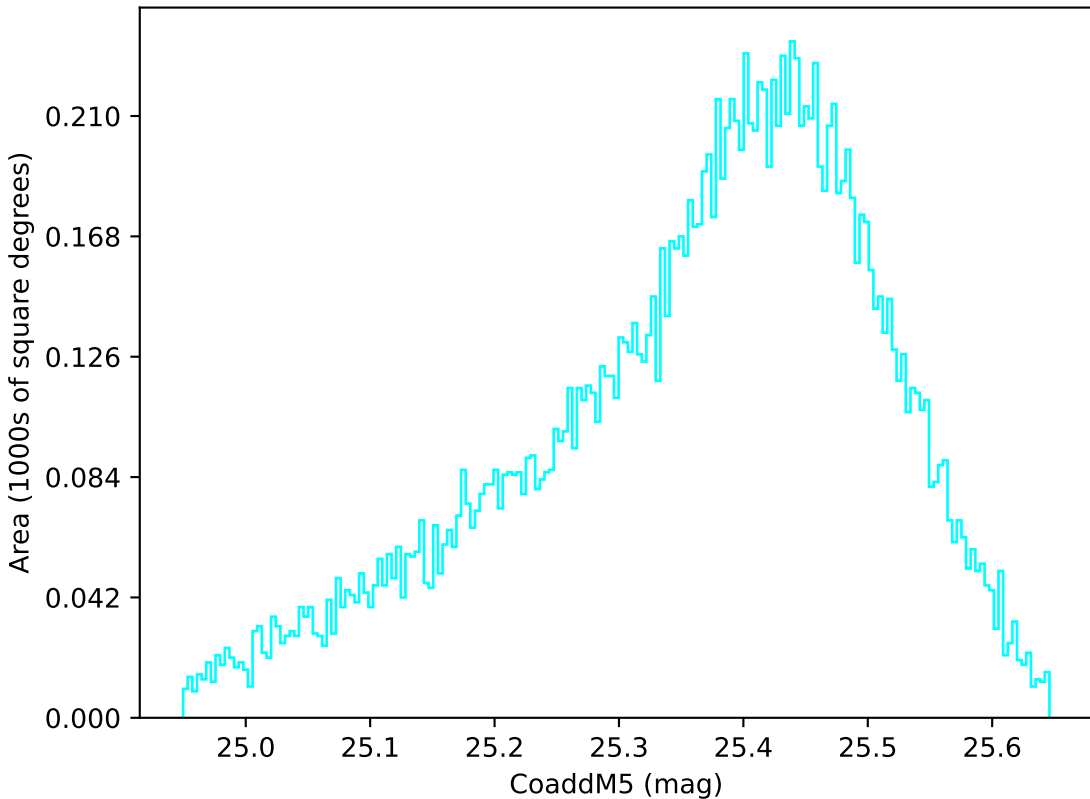
too_elab_r128_d2_griz_v3.4_10yrs WFD u band: CoaddM5
