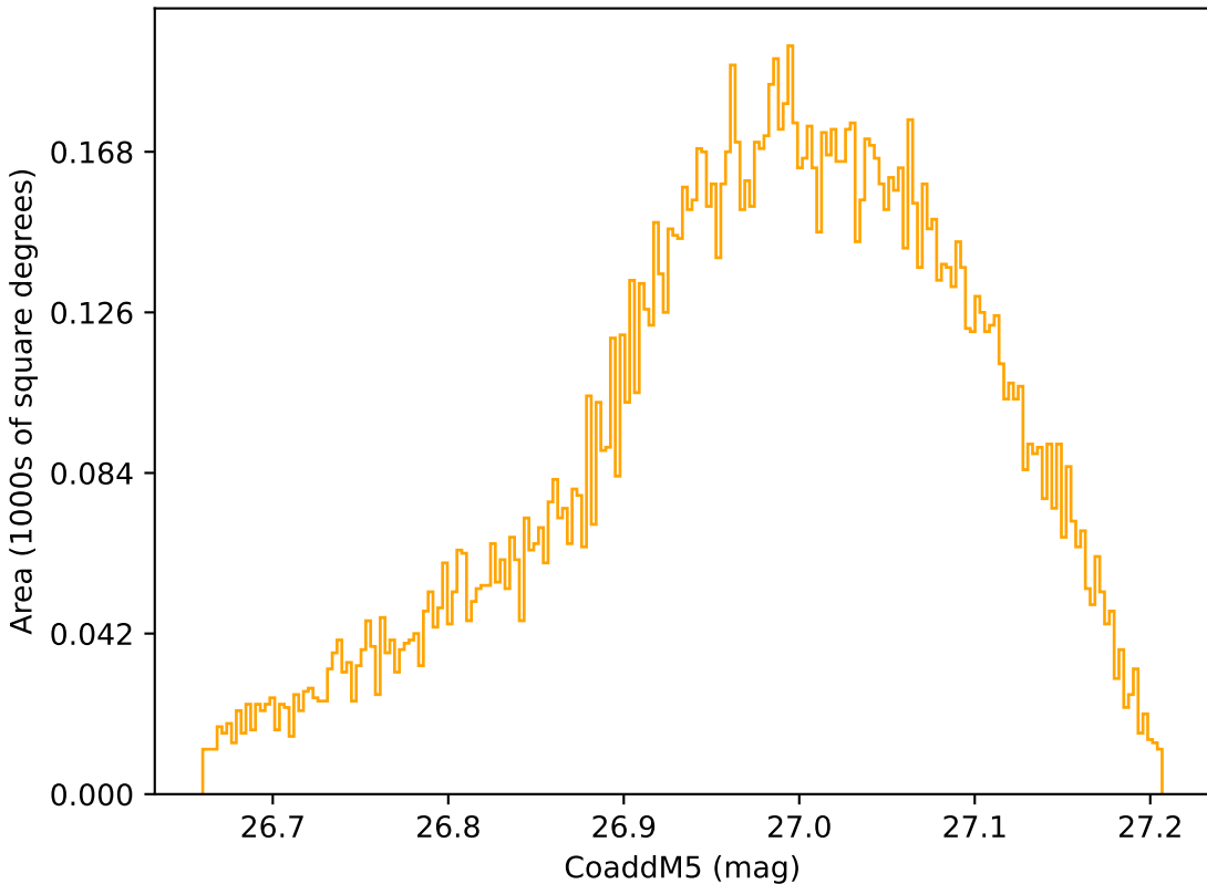
too_elab_r128_d2_griz_v3.4_10yrs WFD r band: CoaddM5
