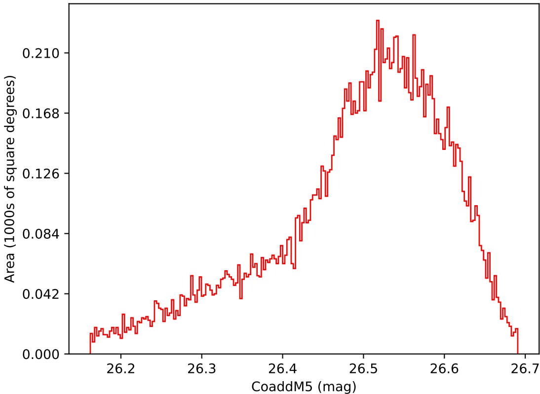
too_elab_r128_d2_griz_v3.4_10yrs WFD i band: CoaddM5
