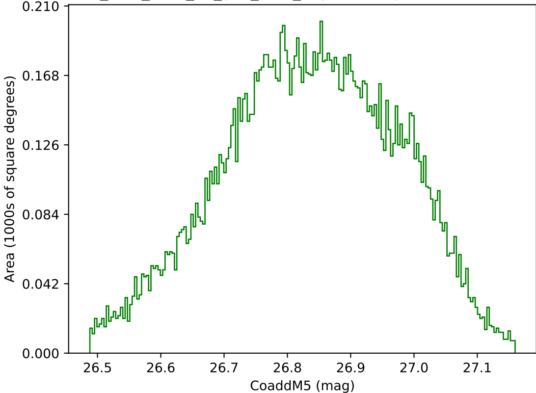
too_elab_r128_d2_griz_v3.4_10yrs WFD g band: CoaddM5
