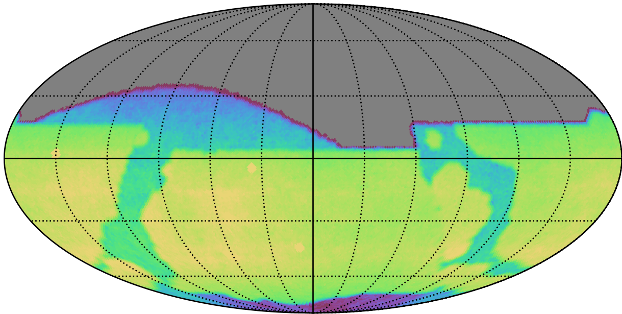
too_elab_r128_d2_griz_v3.4_10yrs All sky r band: CoaddM5
