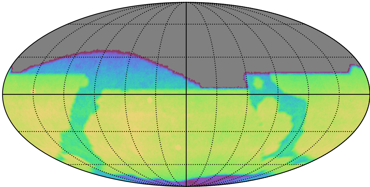
too_elab_r128_d2_griz_v3.4_10yrs All sky i band: CoaddM5
