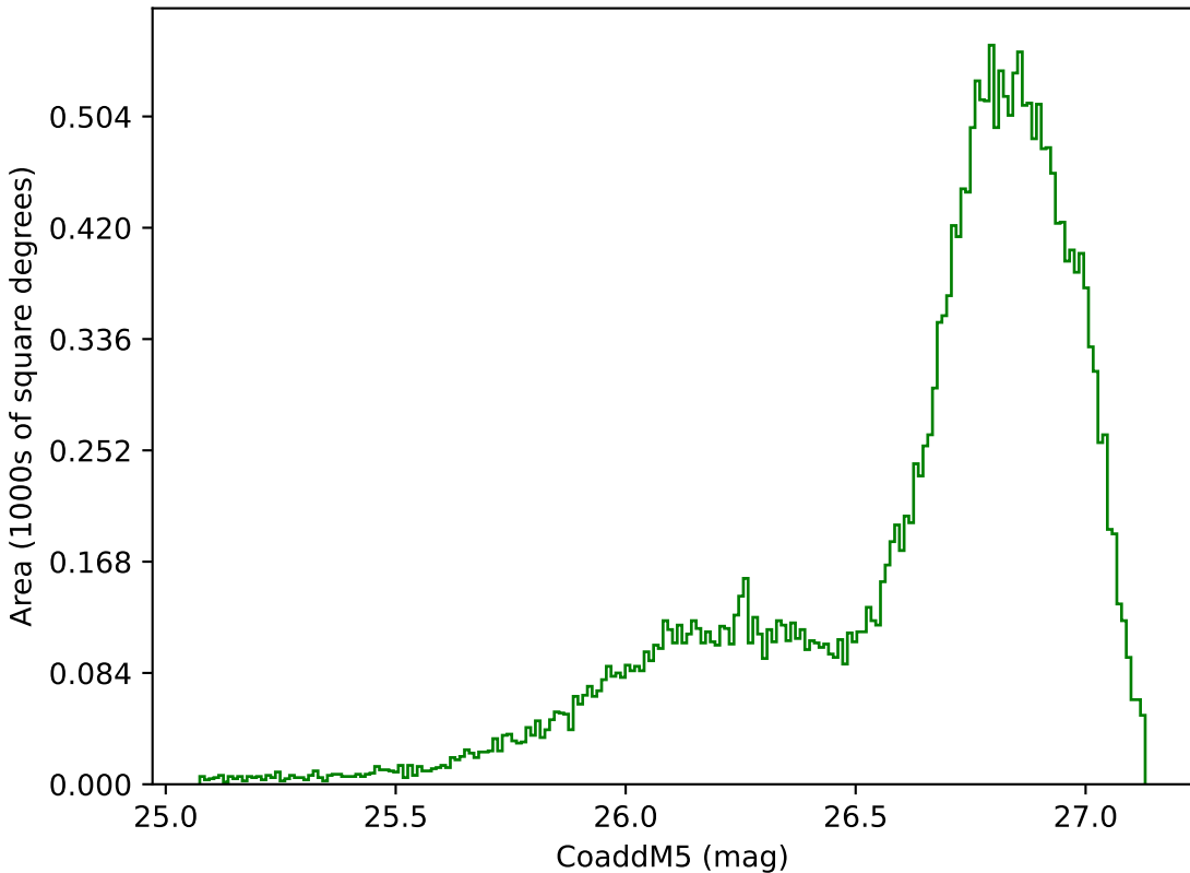
too_elab_r128_d2_griz_v3.4_10yrs All sky g band: CoaddM5
