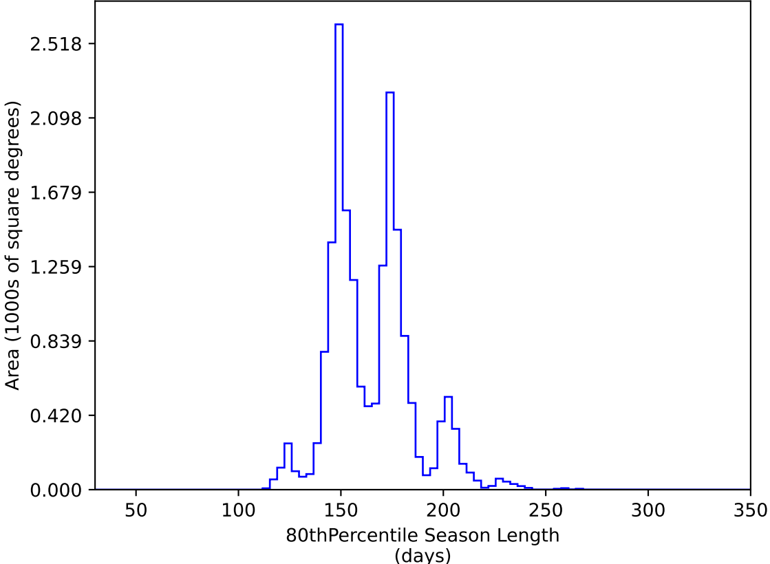
too_elab_r128_d2_griz_v3.4_10yrs WFD y band: 80thPercentile Season Length
