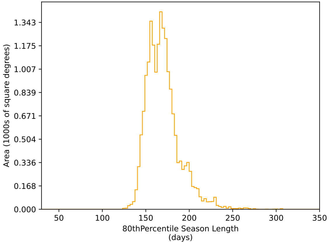
too_elab_r128_d2_griz_v3.4_10yrs WFD r band: 80thPercentile Season Length
