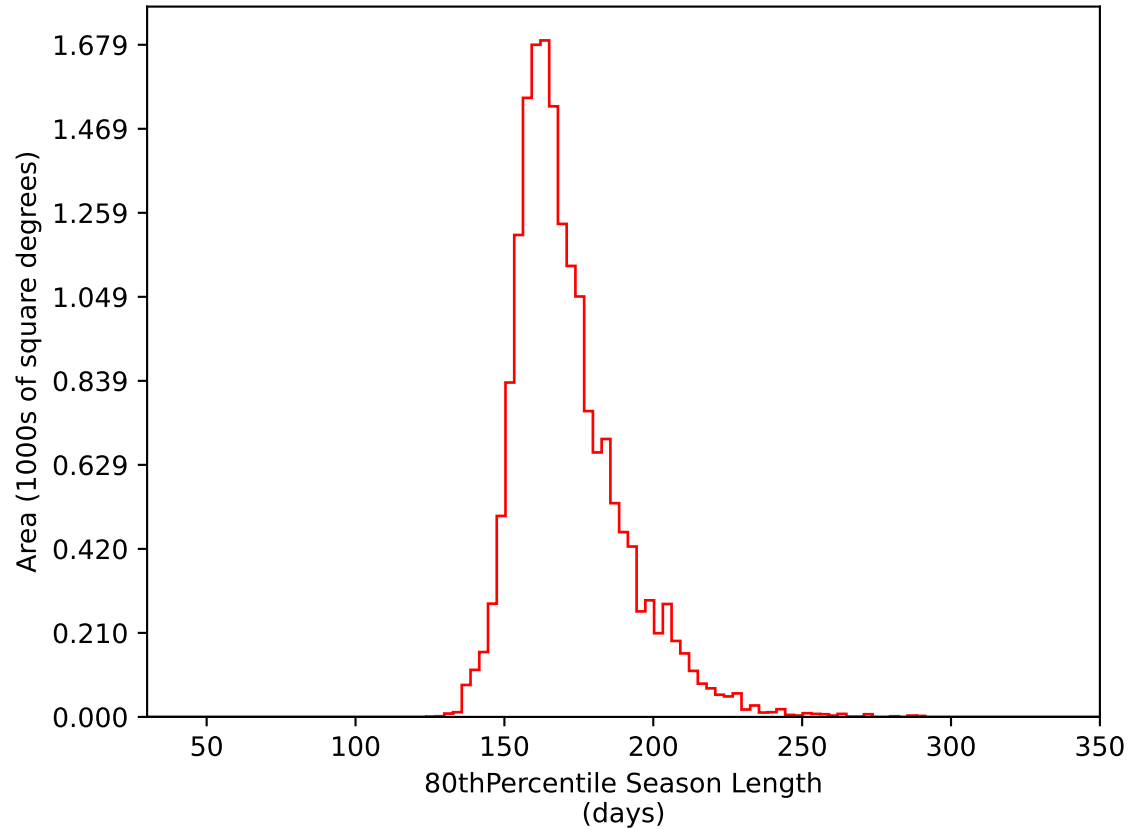
too_elab_r128_d2_griz_v3.4_10yrs WFD i band: 80thPercentile Season Length
