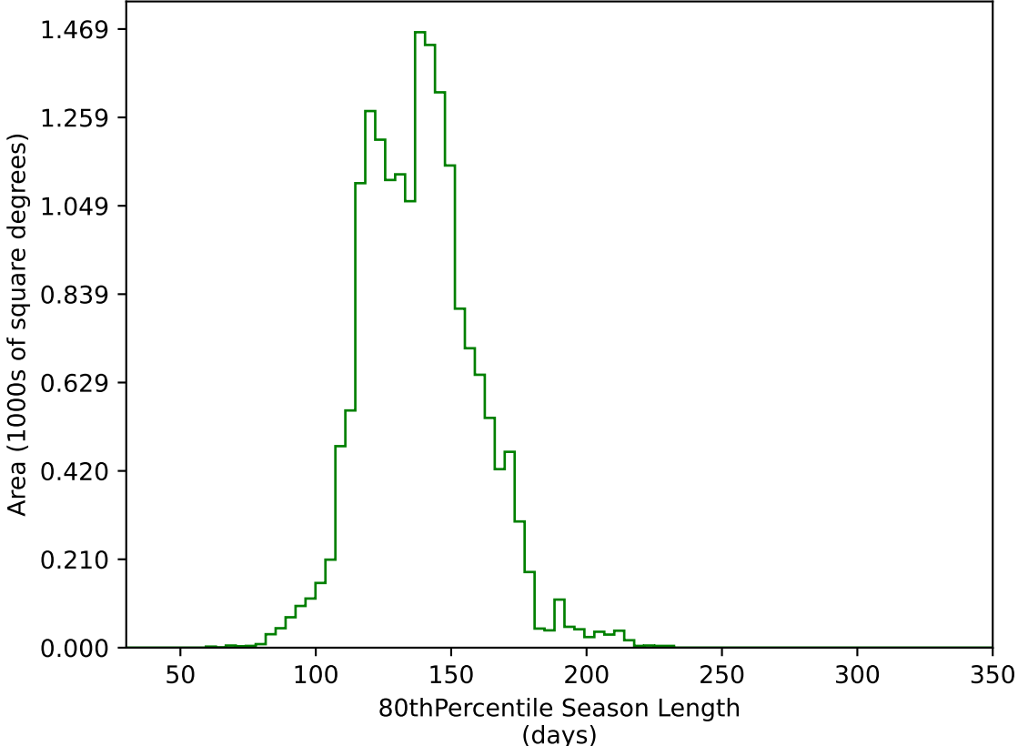
too_elab_r128_d2_griz_v3.4_10yrs WFD g band: 80thPercentile Season Length
