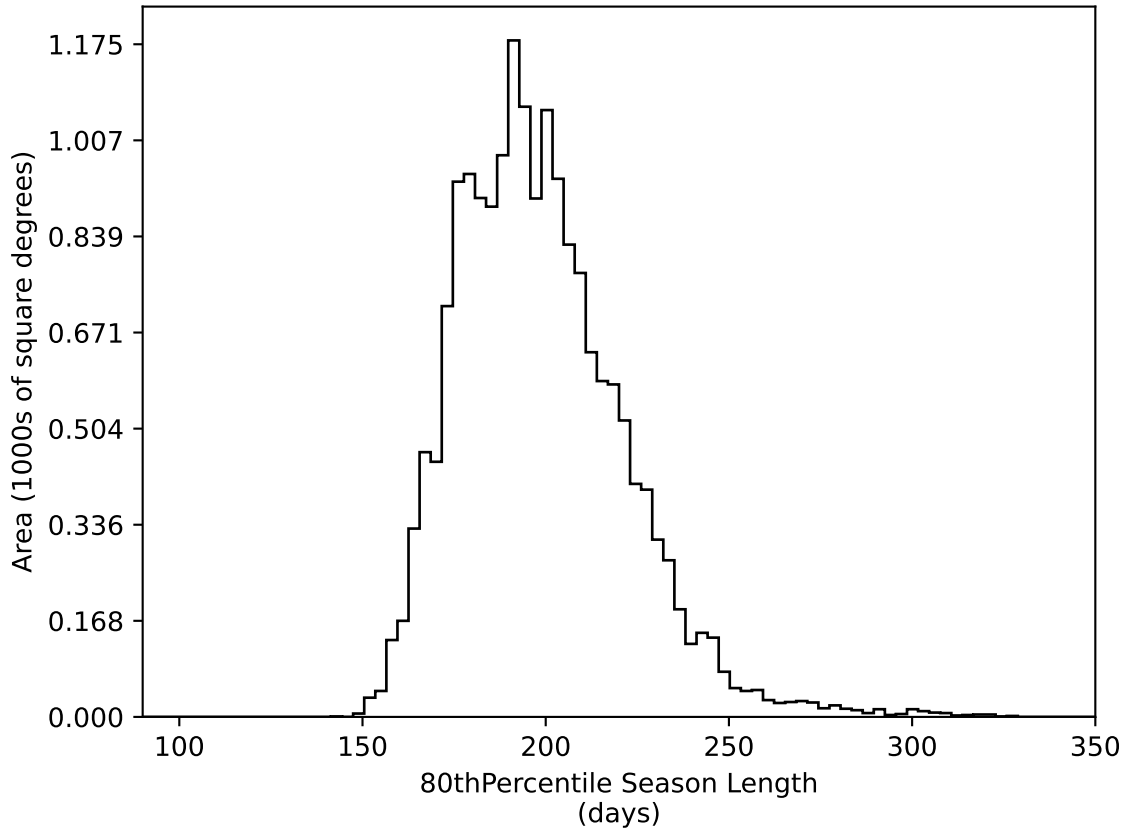
too_elab_r128_d2_griz_v3.4_10yrs WFD all bands: 80thPercentile Season Length
