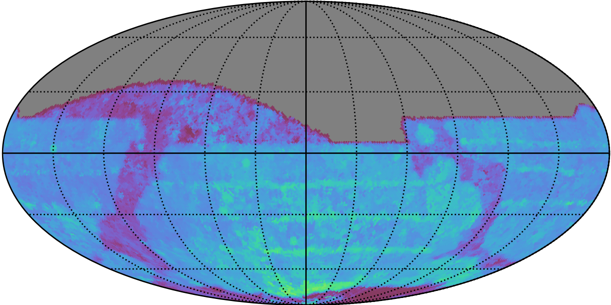
too_elab_r128_d2_griz_v3.4_10yrs All sky z band: 80thPercentile Season Length
