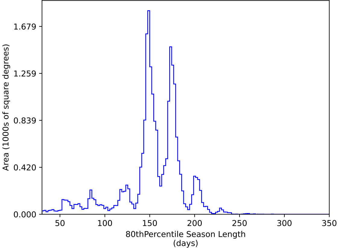
too_elab_r128_d2_griz_v3.4_10yrs All sky y band: 80thPercentile Season Length
