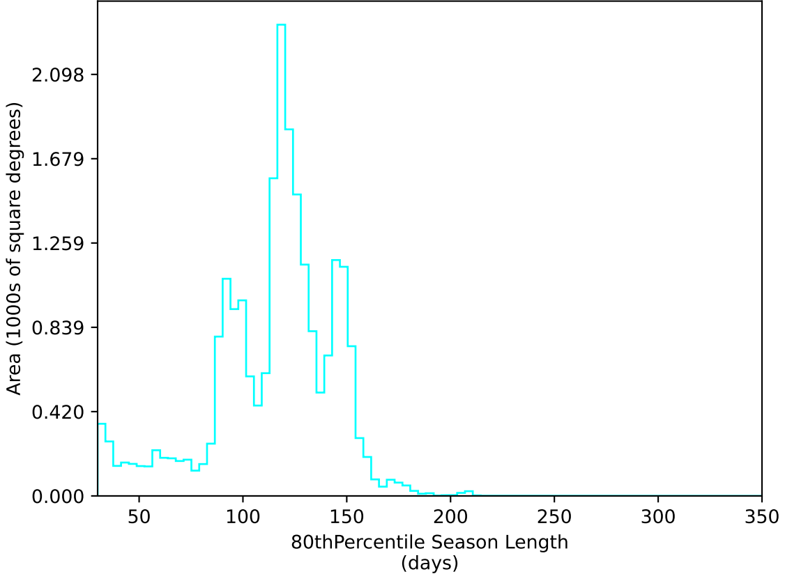
too_elab_r128_d2_griz_v3.4_10yrs All sky u band: 80thPercentile Season Length
